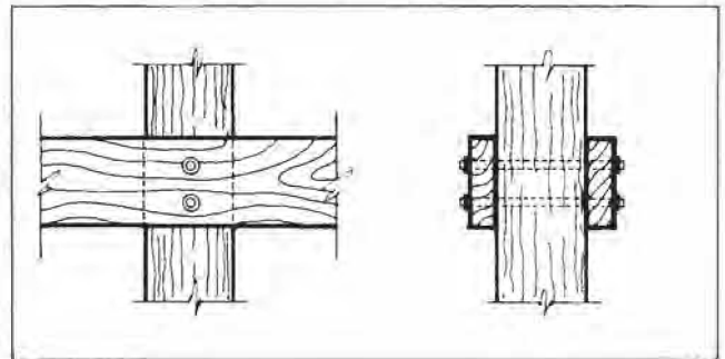
Figure 4.31. Bolted Connection to Round Pole
