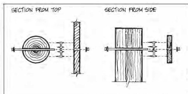
Figure 4.34. Spiked Grid
