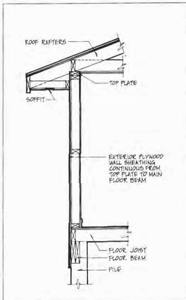
Figure 4.46. Wall Sheathing Tie from Roof to Ceiling
