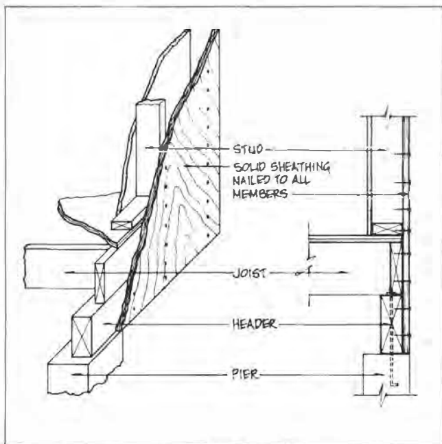
Figure 4.45. Plywood Anchorage
