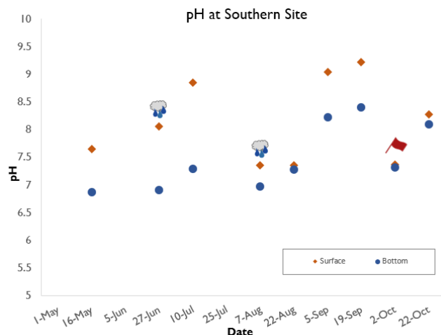
Figure 11 - Surface pH was higher than bottom pH and fluctuated throughout the season.
