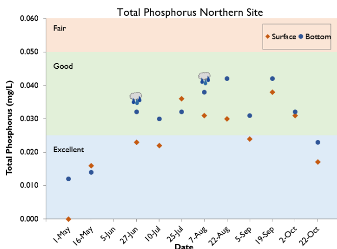
Figure 12 - Surface total phosphorus at the Northern site was considered "Excellent" at the beginning of the season and end of the season, with several results in the "Good" category between July and September. Bottom total phosphorous started in the "Excellent" category, with more results in the "Good" category as the season went on.
