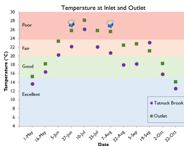
Figure 7 - The temperature at the lake outlet was on average 2.7°C higher than in Tatnuck Brook, demonstrating how much the brook warms after passing through Coes Reservoir.
