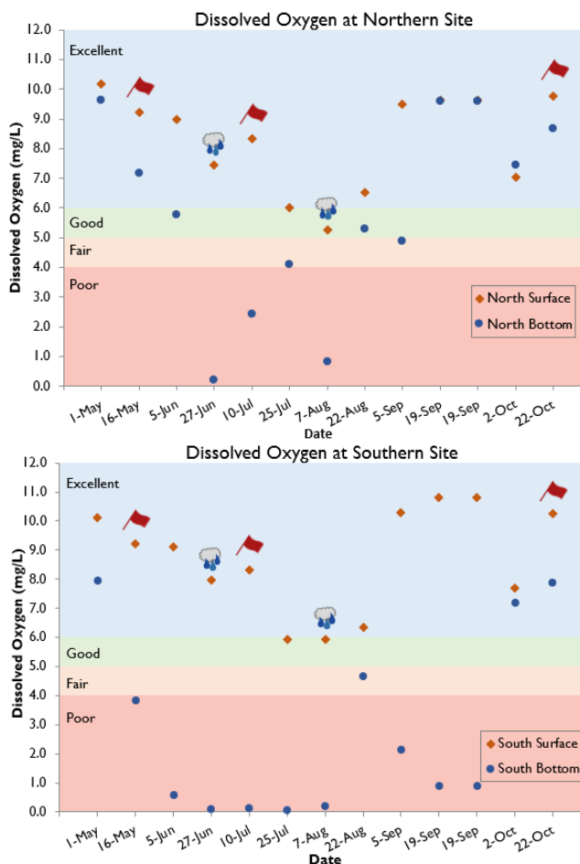
Figures 8 and 9 – At the Northern and Southern sites, dissolved oxygen at the surface was categorized as "Excellent" and "Good" throughout the season. Bottom dissolved oxygen ranged between the "Excellent" and "Poor" categories. "Poor" conditions were more prevalent at the Southern site.
