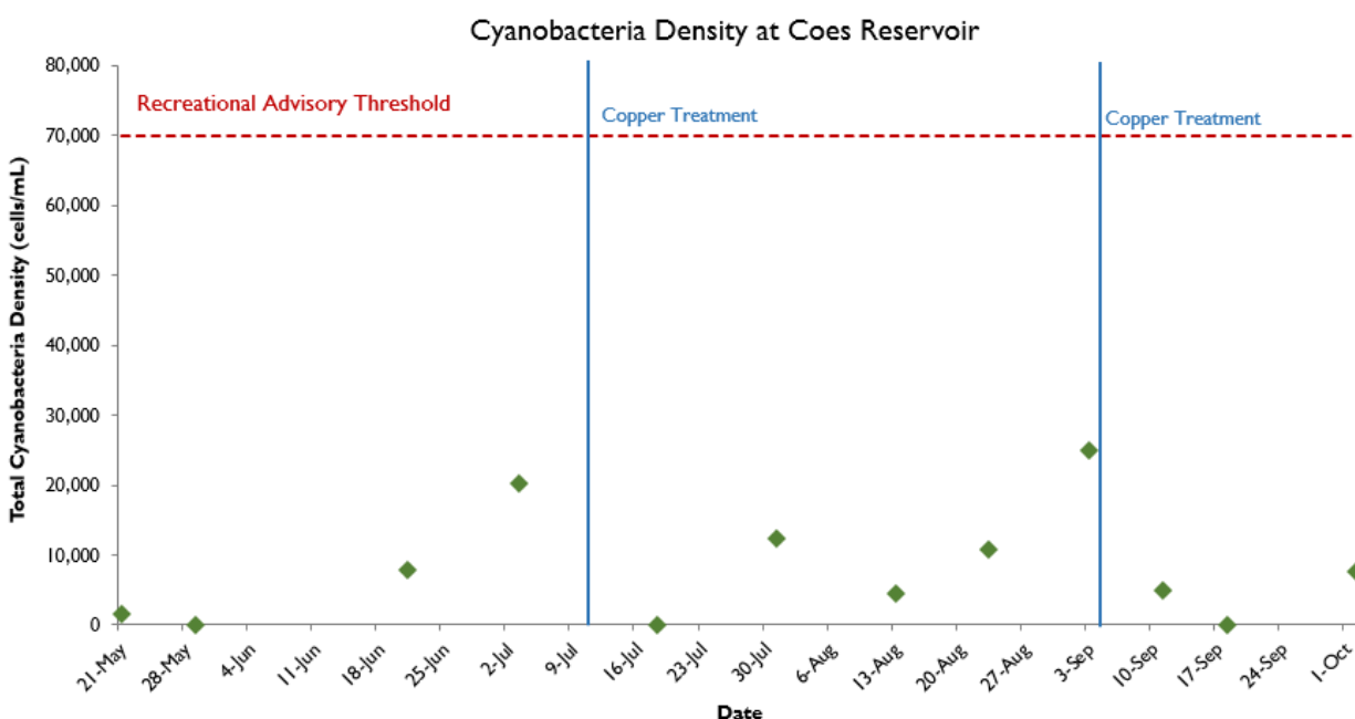
Figure 15 – In 2024 cyanobacteria cell density never exceeded 70,000 cells/mL, the threshold for recreational advisory and lake closure. Copper Sulfate treatments were conducted on 11-Jul and 5-Sep to slow the growth of cyanobacteria.
