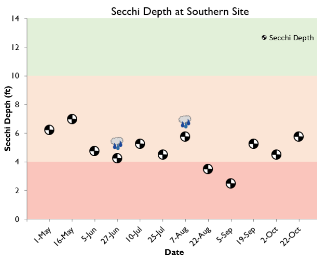
Figure 4 - Secchi depth at the Southern in-lake site was primarily in the range considered "Fair", though two readings were in the range considered "Poor".
