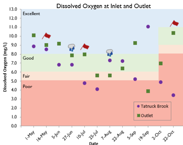
Figure 10 – In Tatnuck Brook and the Coes Reservoir outlet, dissolved oxygen varied widely. Dissolved oxygen at Tatnuck brook was in the range considered “Poor” on four occasions.
