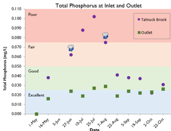
Figure 14 – Total Phosphorous was generally higher at the inlet than the outlet, with 4 of 11 results in the ranges considered “Fair” and “Poor”. Results from the outlet were mostly in the range considered “Excellent”.
