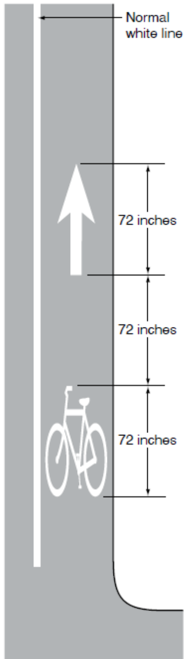
Bike Lane Marking
