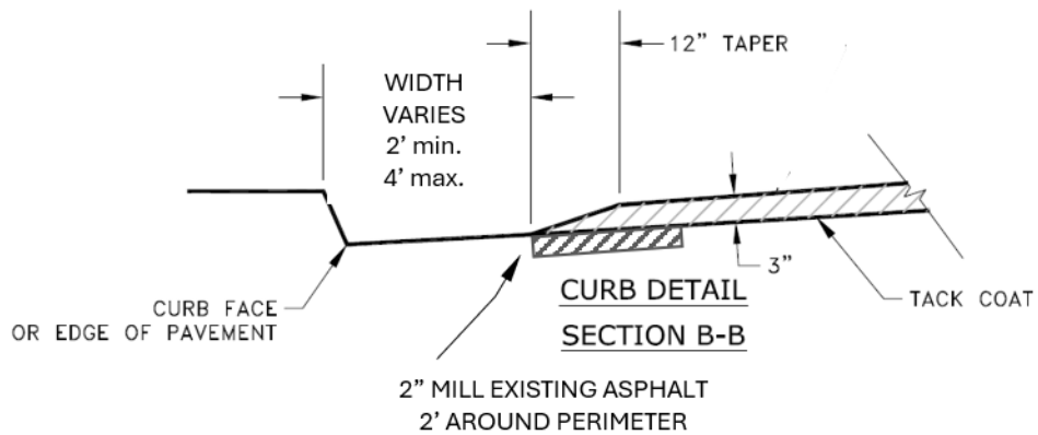
PARABOLIC SPEED TABLE WITH FLAT TOP NOT TO SCALE
