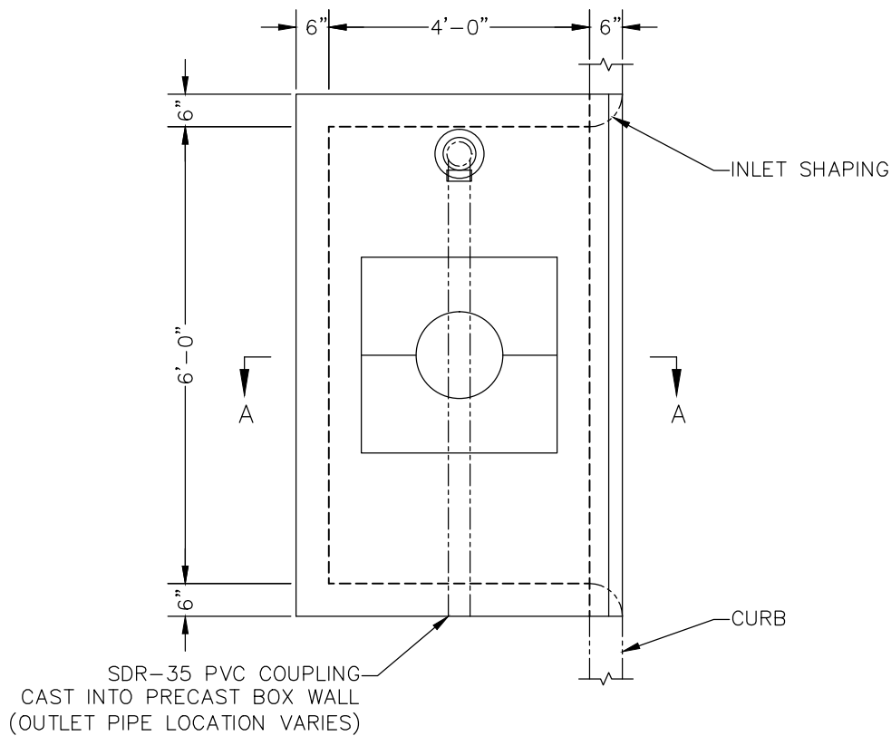
PLAN VIEW
