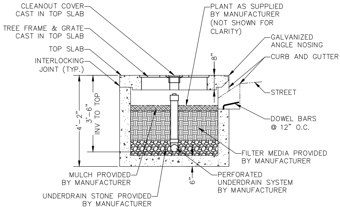
CROSS-SECTION
