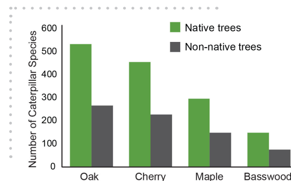
Figure 3: A comparison between the number of caterpillar species native and non-native species of the same genus can support.
