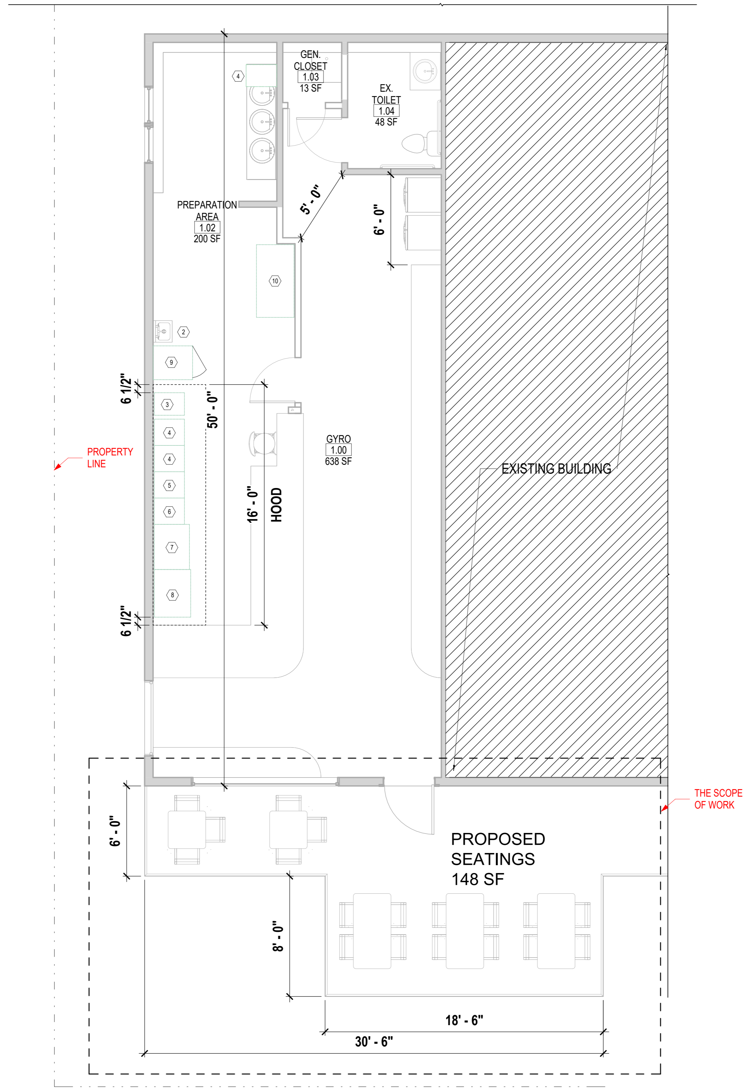
1 1ST FLOOR PROPOSED PLAN 1/4" = 1'-0"
