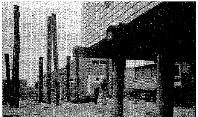
Piles are generally made of wood or prestressed concrete. They often are braced against lateral and shear forces using wood knee and cross bracing, steel rods, and guy wires.
