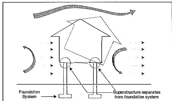
Horizontal wind forces and associated suction (negative forces) on the rear wall can cause an overturning effect.
